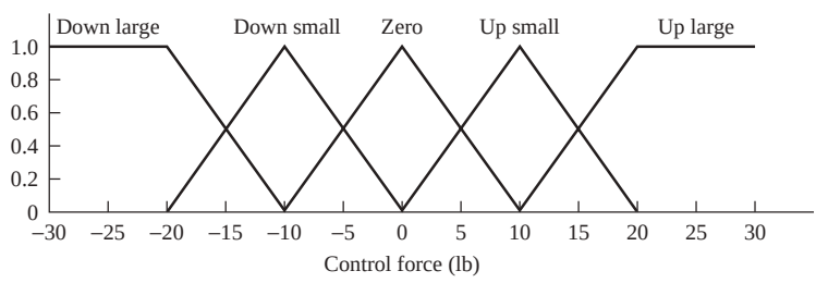
FIGURE 13.11 Control force, f , partitioned.
